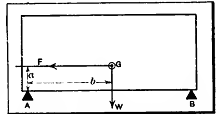
Fig. 2—Illustrating the upsetting and righting moments—G is the center of gravity, F the centrifugal force, W the weight of the car, a the upsetting arm, b the righting arm. A and B are the points of support
